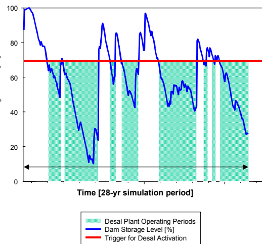
Desalination Plant Operating Rule 70% water storage trigger level
